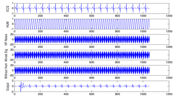
Fig.4 Original ECG Signal with HUM and High Frequency Noise Simulation by Notch Filter
