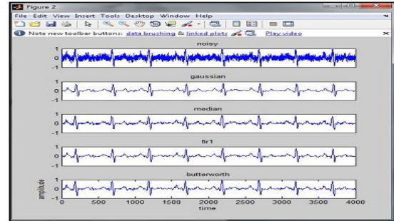
Fig.3 Results of Gaussian, median, FIR and Butterworth filters
